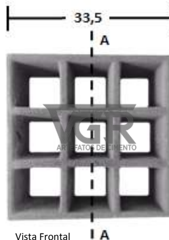
Vista Frontal
